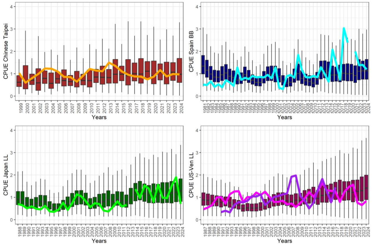
Figure 19.5.2 CPUE trajectories simulated in the MSE (boxplots) and updated standardized CPUEs (lines). Chinese Taipei-LL (orange), Spain-BB (blue), Japan-LL (green) and USA-LL (pink) were all updated to 2024, and Venezuela-LL (purple) has not been updated since 2017.
