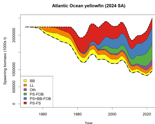
Figure 2. Impact plots represent the relative impact of each gear on the spawning biomass of the stock. Coloured areas represent model predicted increases in spawning biomass when catches of each gear are eliminated from the historical catches. The estimated unfished spawning biomass (dotted line) varies with recruitment deviations. The historical SSB trajectory, estimated by the stock assessment model, is indicated with a dashed line. The code PS FOB represents the purse seine fisheries operating on FOB/FADs. The code PS+BB-FOB reflects that these purse seine fleets have operated in association with baitboats (BB) in the past. The free school refers to the purse seine operations on free school banks.
