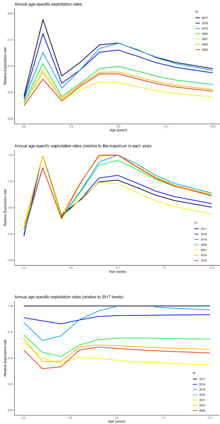
Figure 19.30.3 Patterns in recent estimates of age-specific exploitation rates of Atlantic bigeye tuna estimated from the reference case model. ( Top panel ) the 'raw' estimates; ( middle panel ) estimates scaled within each year to the age with the highest exploitation rate; and ( bottom panel ) estimates scaled within each age to the value for that age in 2017.
