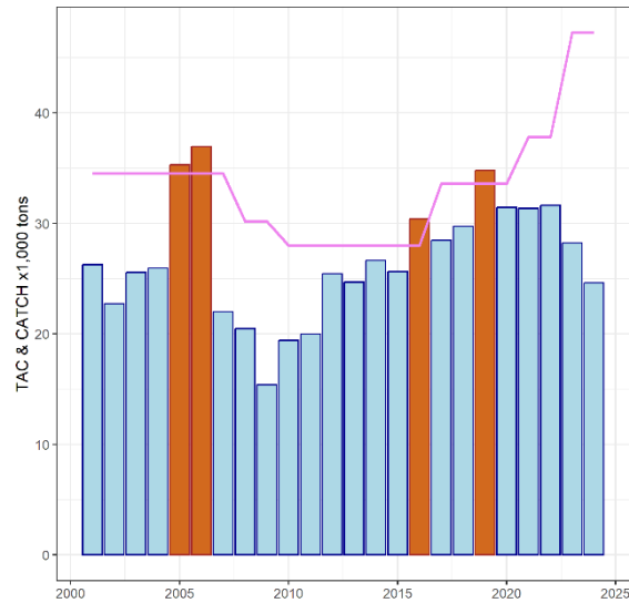
Figure 19.5.1 ALB-N reported catch (Task 1NC, bars) and TAC (solid line). Orange bars indicate years when the catch exceeded the TAC. Note that TAC was established with the ALB-N HCR or the MP started in 2018.
